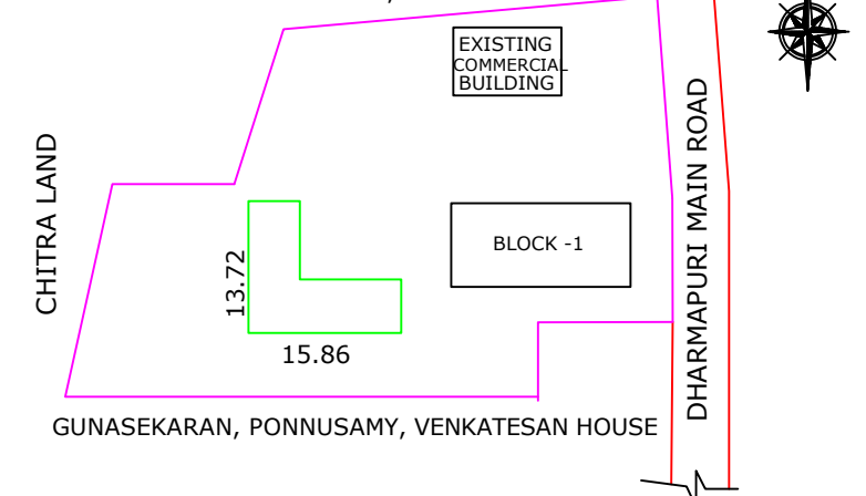
SITE CUM PRO.GROUND FLOOR
