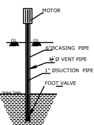
SEC. OF BOREWELL
