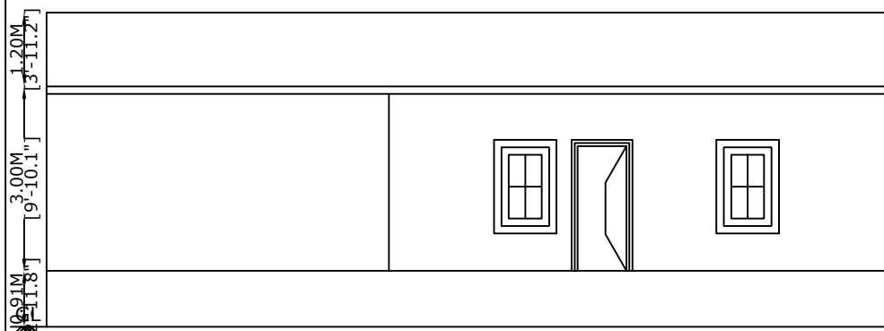
FRONT ELEVATION
