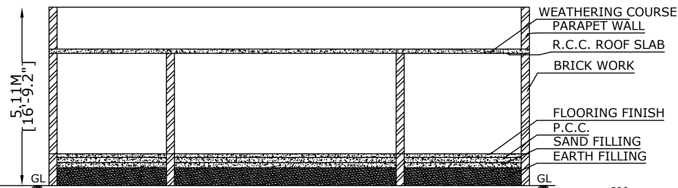
SECTION ON XX
