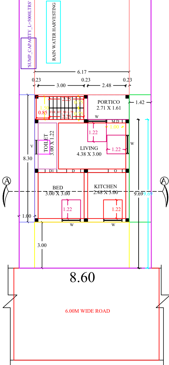
SITE CUM GROUND FLOOR PLAN
