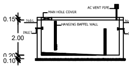
PLAN OF SEPTIC TANK
