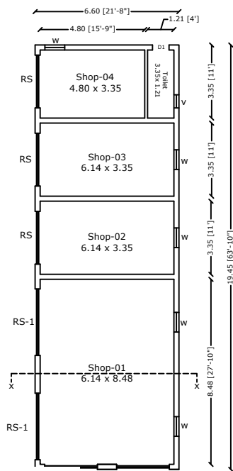
FLOOR PLAN
