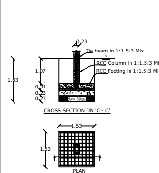
COLUMN FOUNDATION DETAILS:-
