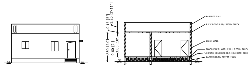
FRONT ELEVATION
