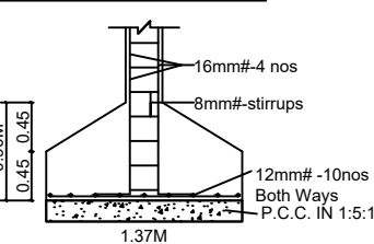
FOOTING DETAILS
