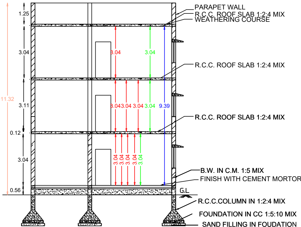
SECTION SS SCALE : 1/100
