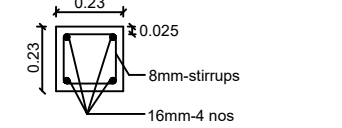
COLUMN DETAILS COLUMN SIZE: 0.23X0.23
