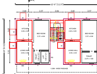
SECOND FLOOR PLAN SCALE 1:100
