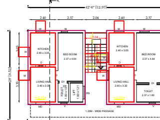
THIRD FLOOR PLAN SCALE 1:100
