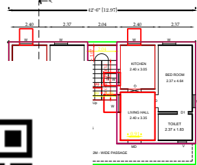
FLOOR PLAN SCALE 1:100
