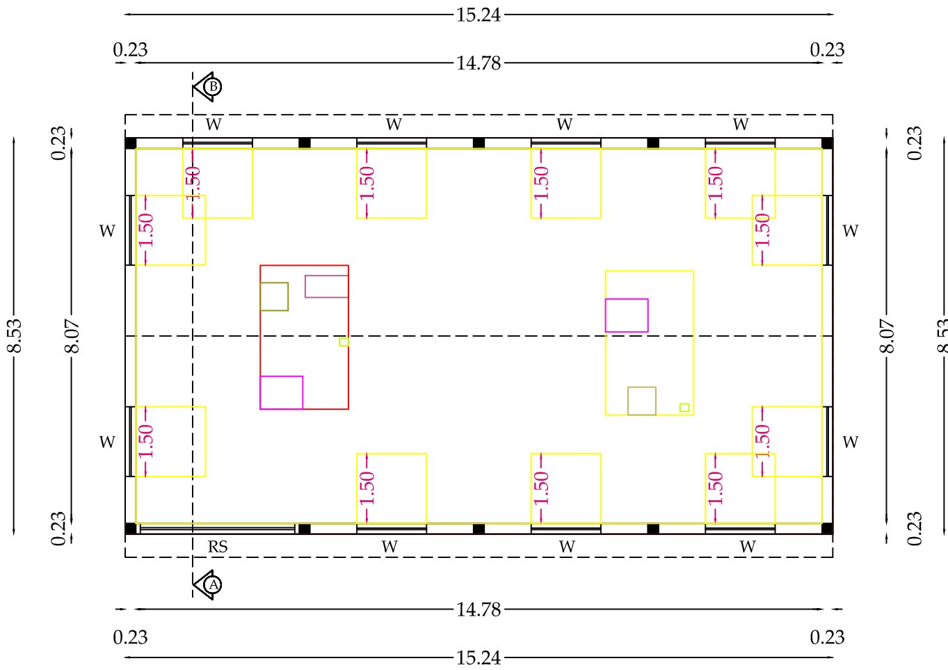
PLAN
