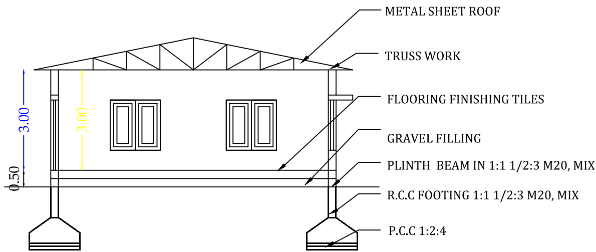
SECTION A TO B
