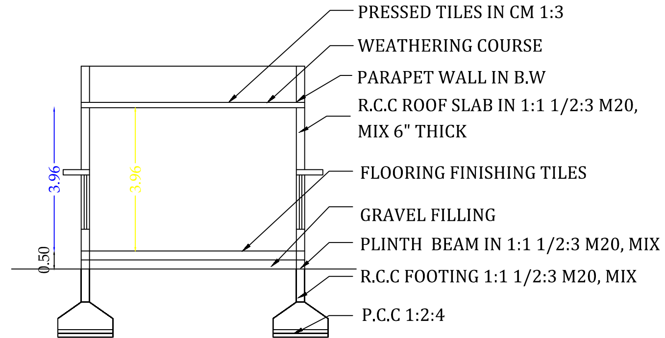
SECTION A TO B
