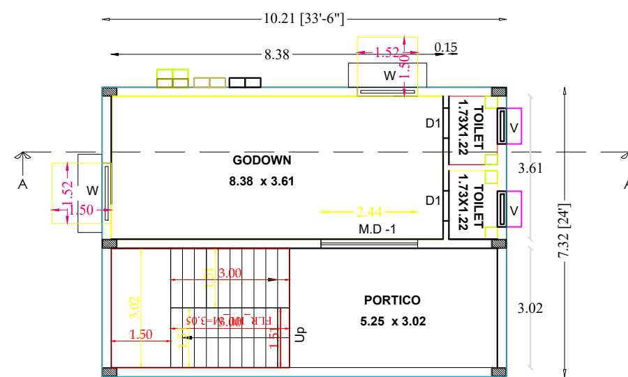
GROUND FLOOR PLAN SCALE = 1:100 GODOWN BUILDING
