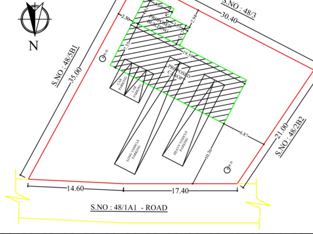
SITE PLAN (1:100)
