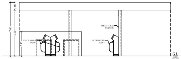
FRONT ELEVATION
