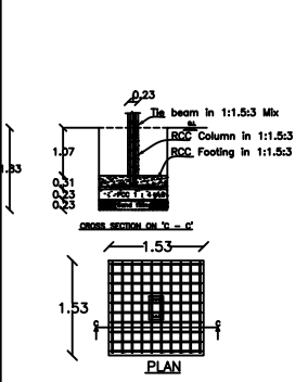
COLUMN FOUNDATION DETAILS:-
