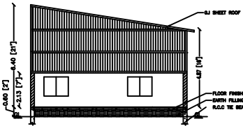
SECTION ON X-X
