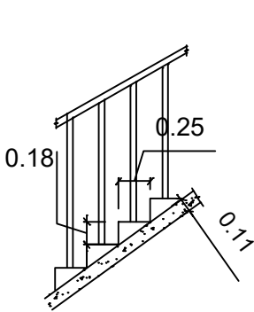
STAIRCASE DETAILS:-
