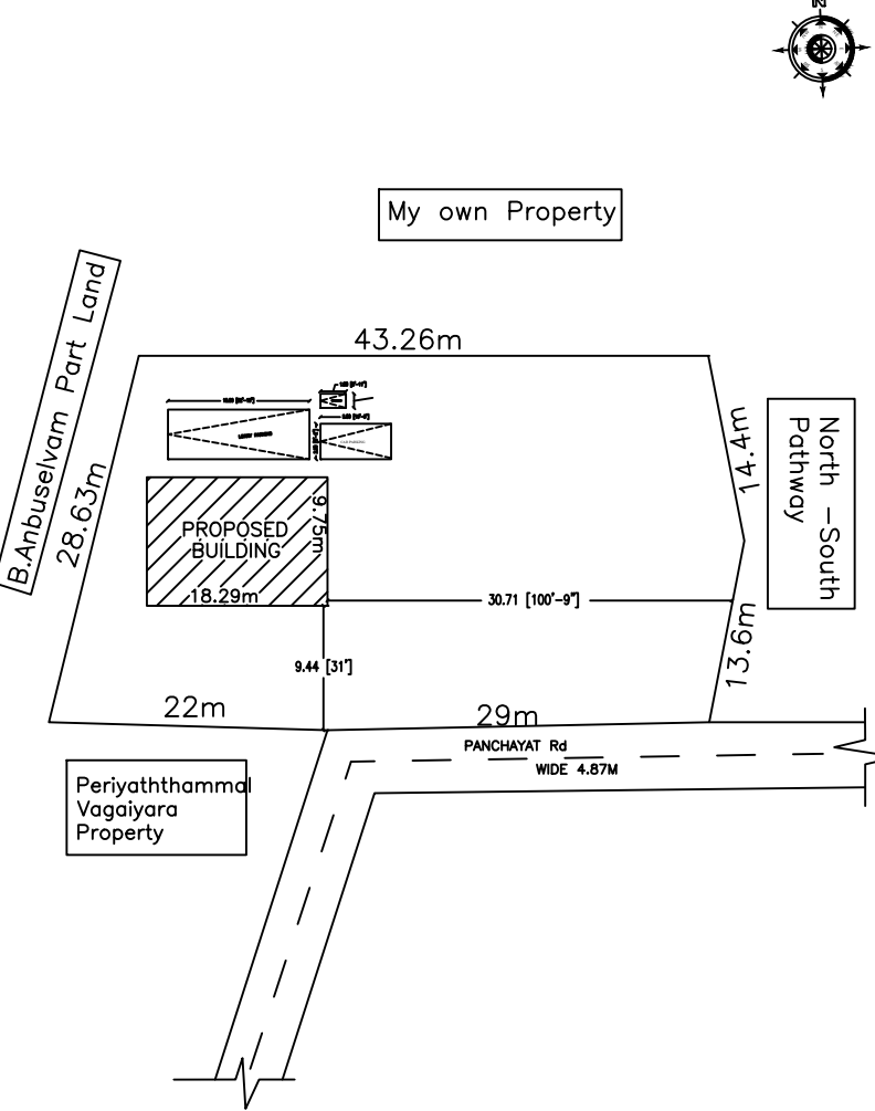
TAKEN SITE PLAN:- (SCALE 1:100)
