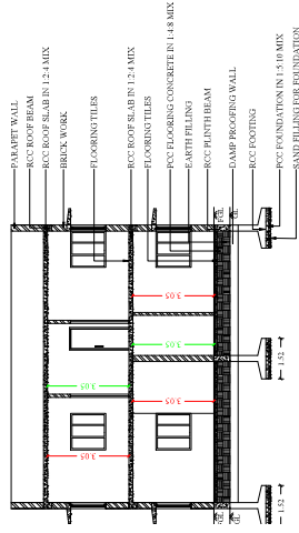
SECTION ON-AA
