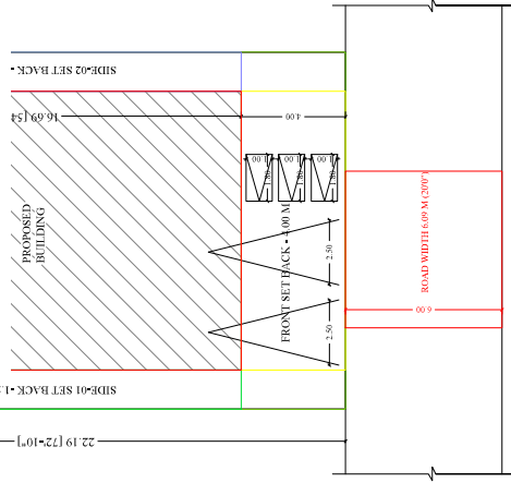
SITE PLAN
