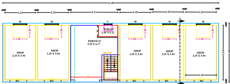
GROUND FLOOR
