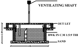
SEPTIC TANK
