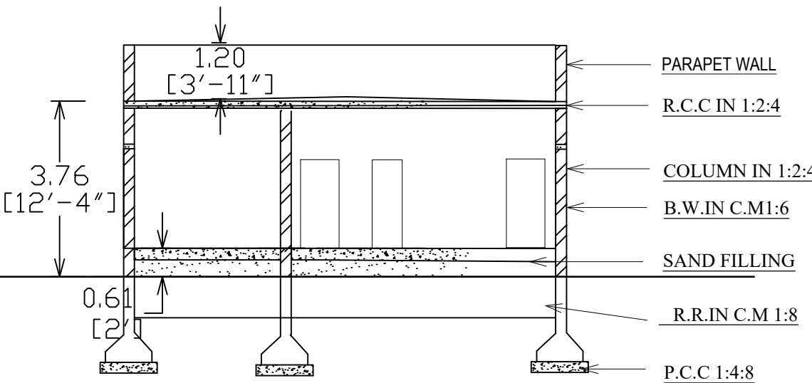
SECTION ON-AA
