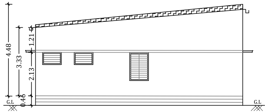
FRONT ELEVATION ON A-A
