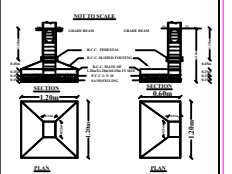
TYP.DET. COLUMN FOOTING
