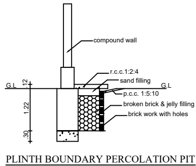
PLINTH BOUNDARY PERCOLATION PIT
