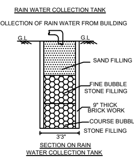
SECTION ON RAIN WATER COLLECTION TANK
