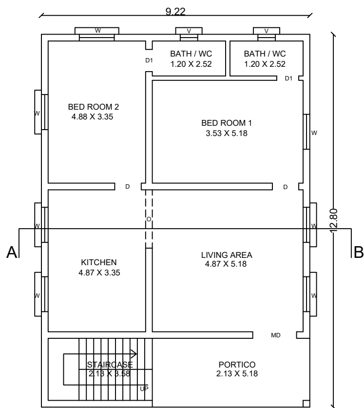
PRO GROUND FLOOR ( EAST FACING )
