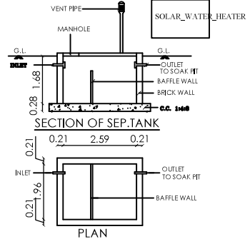
PLAN SEPTIC TANK
