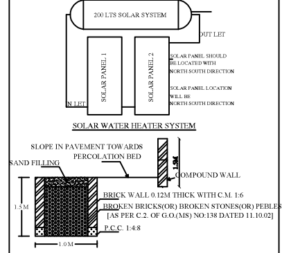
SECTION OF RAIN WATER PERCOLATION BED
