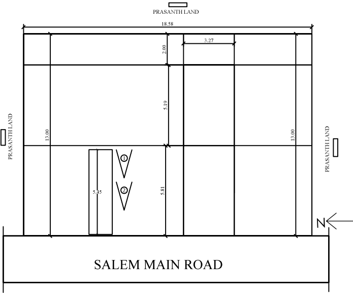
FOUNDATION DETAILS
