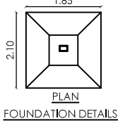
FOUNDATION DETAILS
