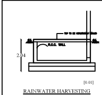
RAINWATER HARVESTING
