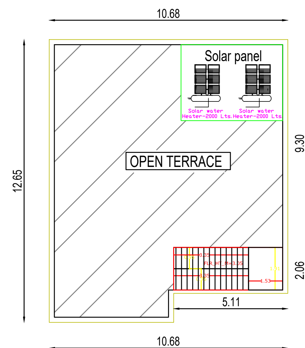
PROPOSED TERRACE FLOOR PLAN (Scale 1:100)
