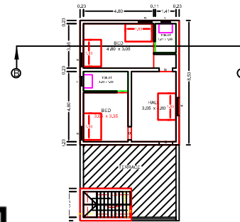
FLOOR-FIRST
