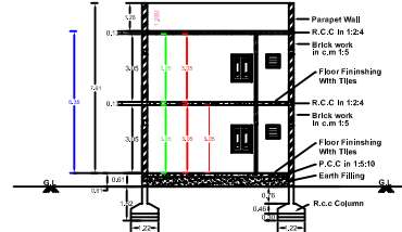
Section on 'BB'
