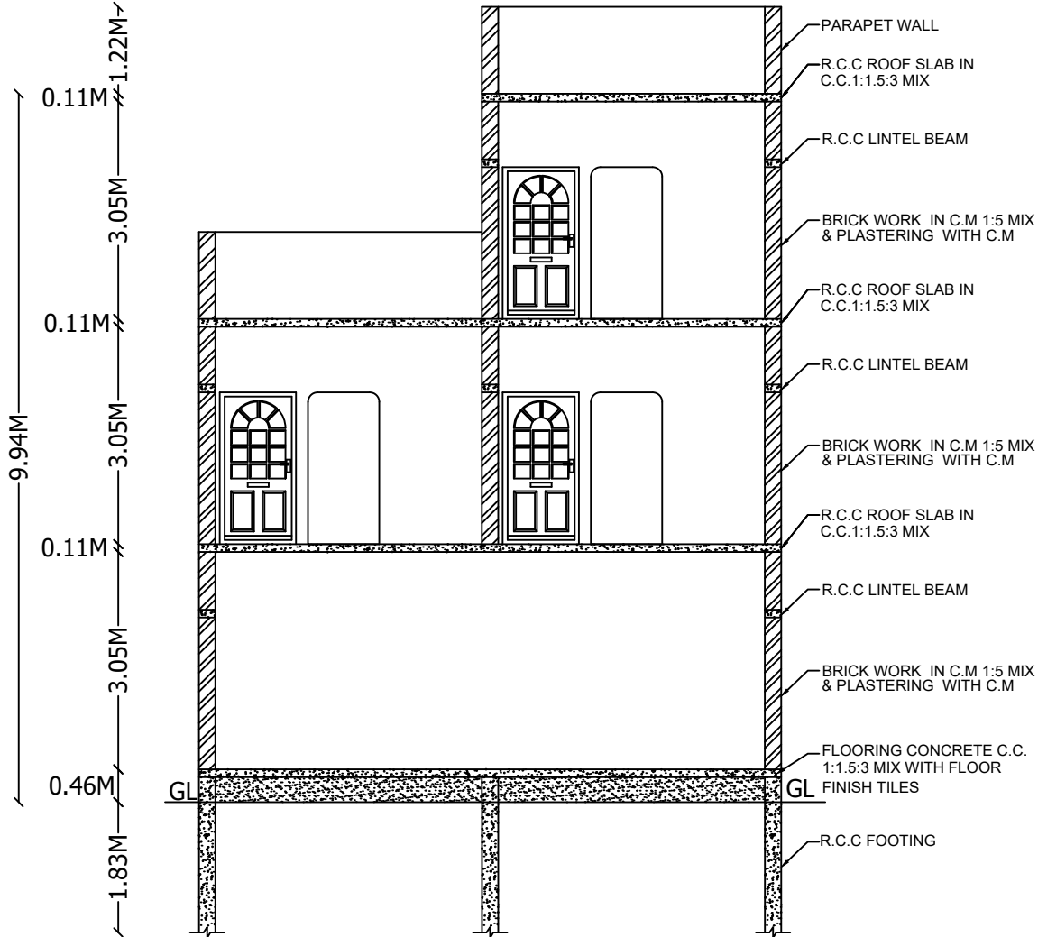
SECTION AA
