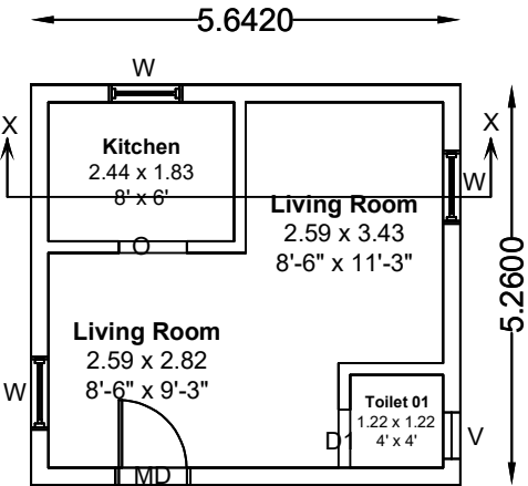
SITE CUM PRO.GROUND FLOOR
