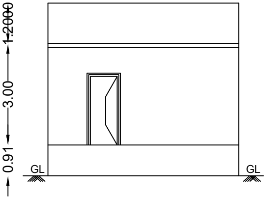
FRONT ELEVATION
