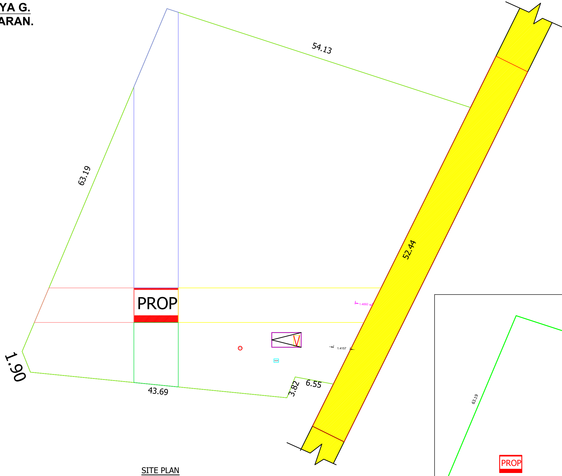
SITE PLAN
