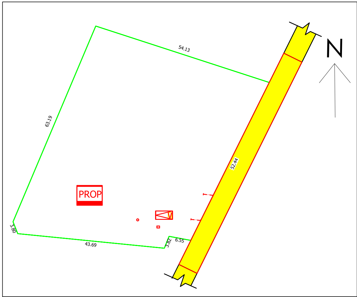
KEY PLAN
