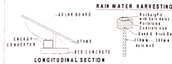
SOLAR SYSTEM
