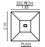
FOUNDATION DETAILS
