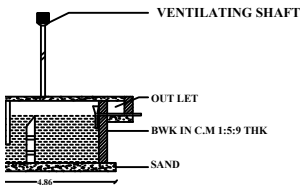
SECTION OF THE SEPTIC TANK
