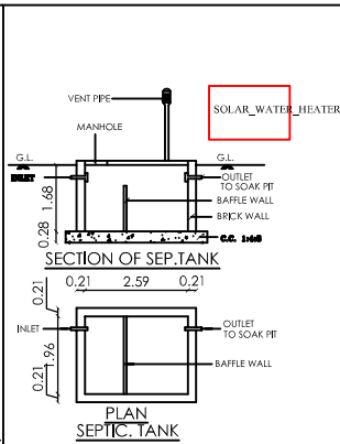
PLAN SEPTIC TANK
