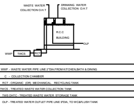
FLOW DIAGRAM OF WASTE WATER RECYCLING & REUSE
