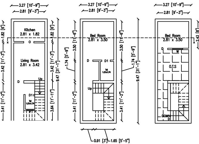
FIRST FLOOR PLAN SECOND FLOOR PLAN
