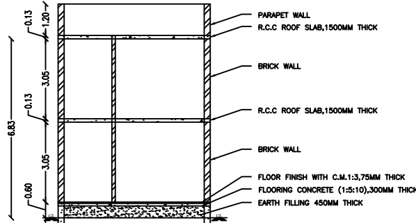
SECTION ON X-X
