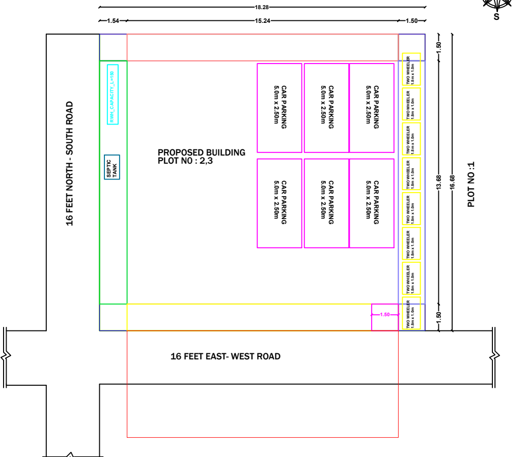
SITE PLAN
