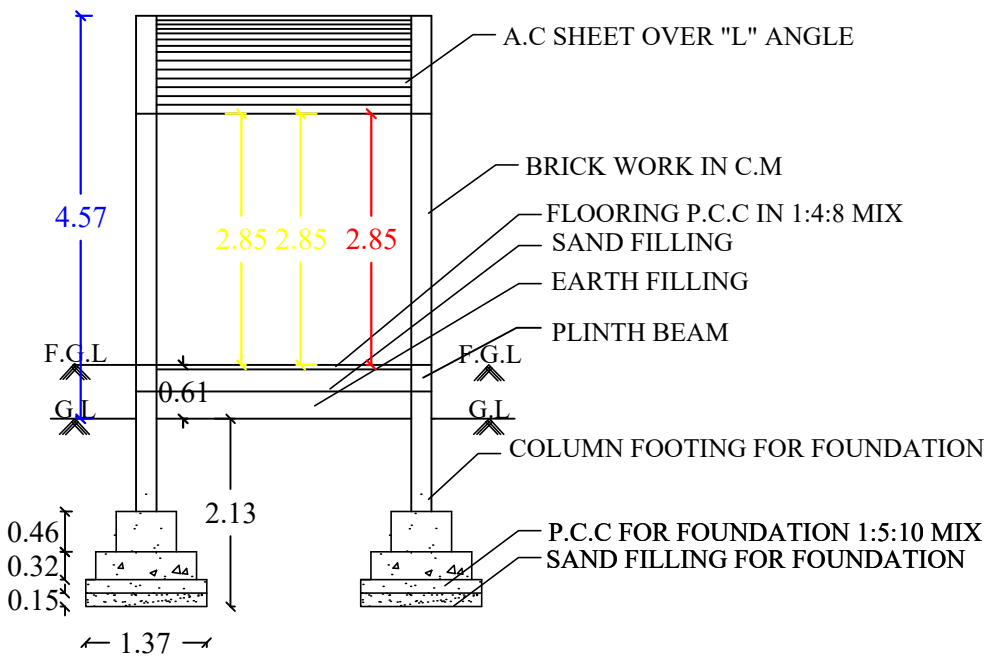
SECTION ON-AA
