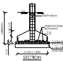
SECTION
