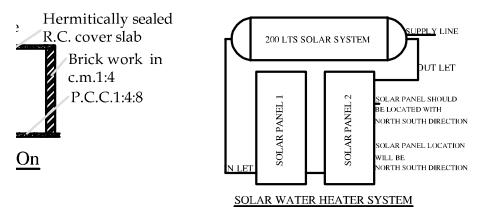
SOLAR WATER HEATER SYSTEM
