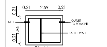
SEPTIC. TANK
