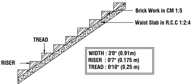
STAIRCASE DETAILS
