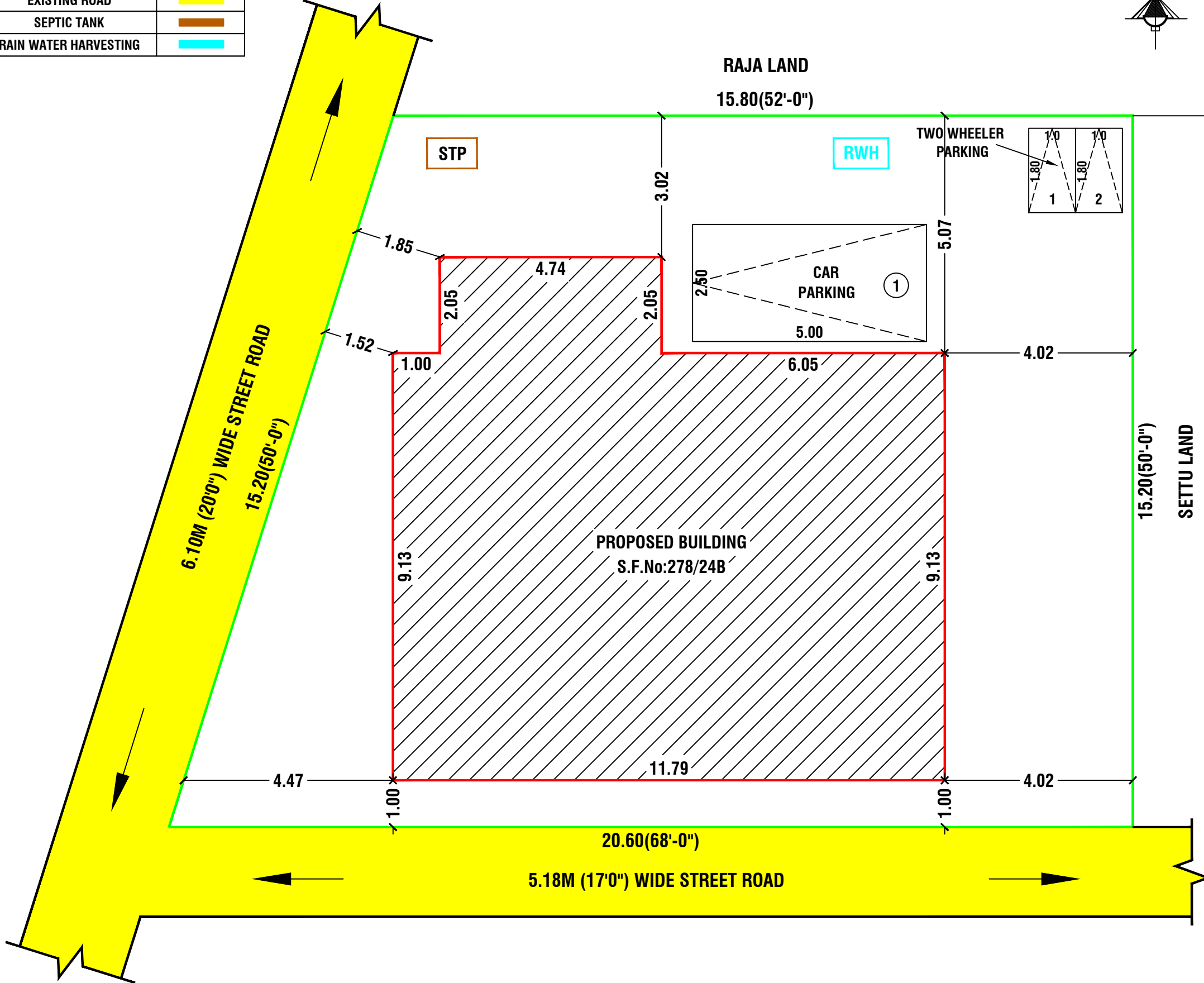
SITE PLAN SCALE 1:100 -- As Per FMB & Document
