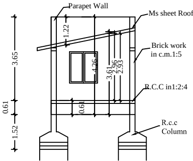
CROSS SECTION-AA
