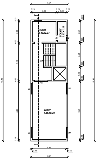
PROPOSED FIRST FLOOR PLAN
