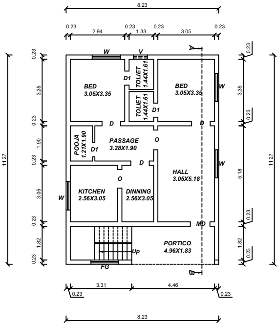
FLOOR PLAN PLAN ]
