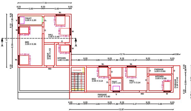
PRO.SECOND FLOOR
