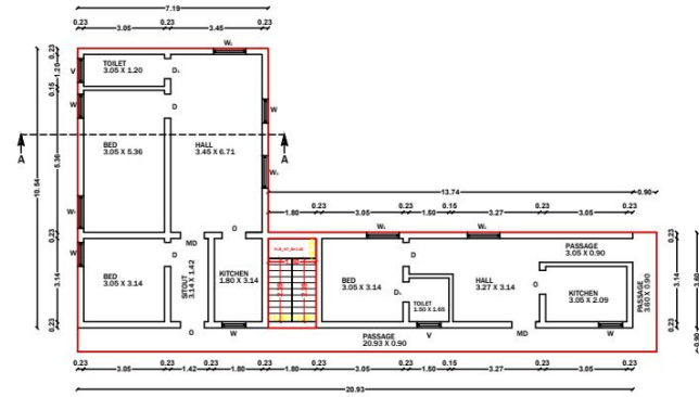
EXI.FIRST FLOOR
