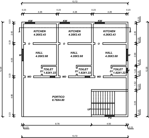
EXISTING GROUND FLOOR PLAN ( NORTH FACING PLAN )
