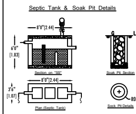
Septic Tank & Soak Pit Details
