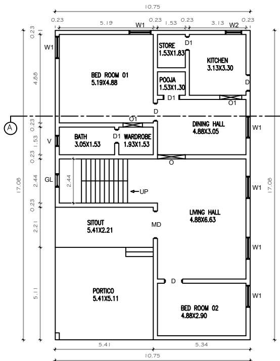
PROPOSED OF GROUND FLOOR PLAN
