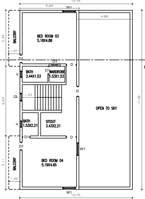
PROPOSED OF FIRST FLOOR PLAN
