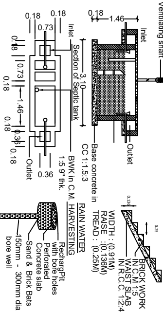
SEPTIC TANK DETAIL
