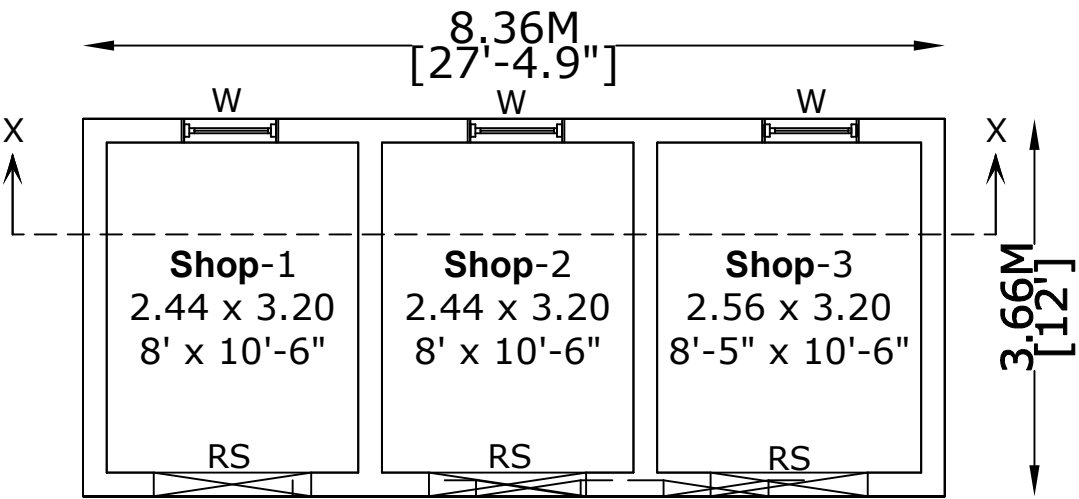
SITE CUM PRO.GROUND FLOOR
