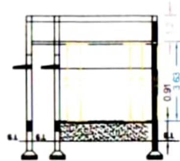
SECTION - 'X-X'
