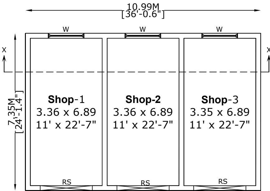
SITE CUM PRO.GROUND FLOOR
