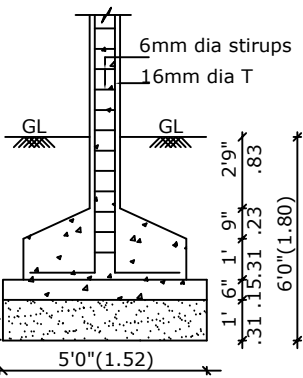
COLUMN FOUNDATION DETAIL
