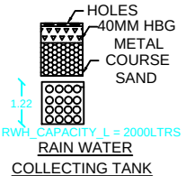
RAIN WATER COLLECTING TANK
