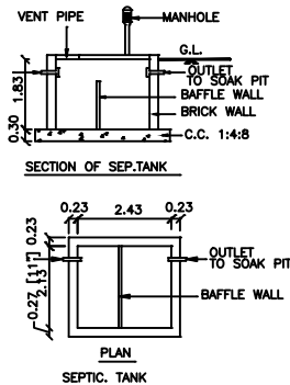
SEPTIC TANK
