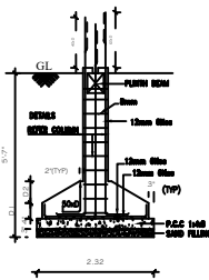
FOUNDATION DETAILS
