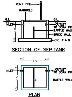
SEPTIC TANK
